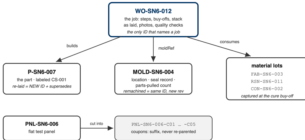
Figure 1: Figure 1. The record graph for one job: the work order builds a part, points at a mold record, and consumes lots; a panel's coupons are suffixes, never records of their own. The rules under the boxes are §4.1's, drawn where they apply.
